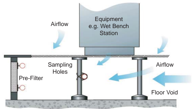
Sample pipe in the floor void beneath a raised access floor will capture smoke as it is carried by the airflow.
